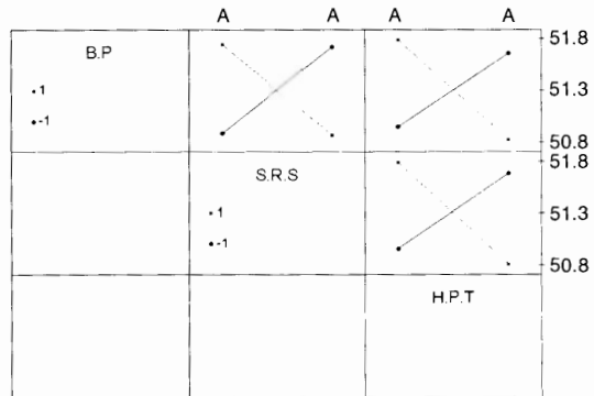
Figure 13 Interaction plot for analysis B
