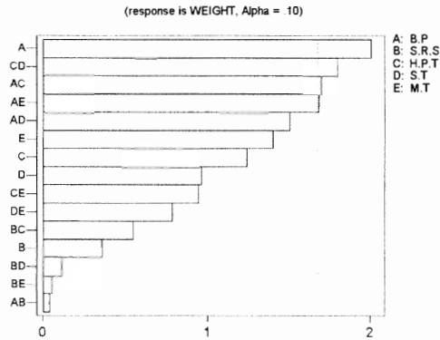
Figure 8 Pareto chart of standardized effect
