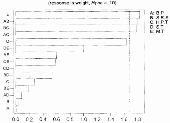
Figure 12 Pareto chart of standardized effect
