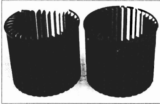
Figure 5 Example of short-shot defect
