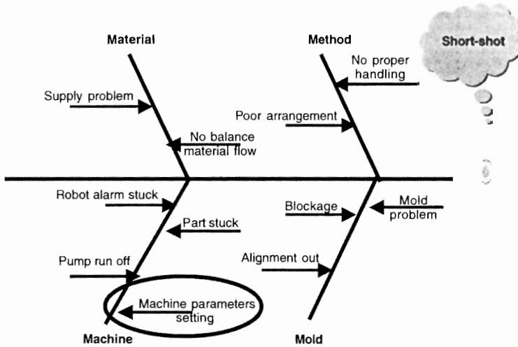
Figure 6 Cause and effect diagram for short-shot problem
