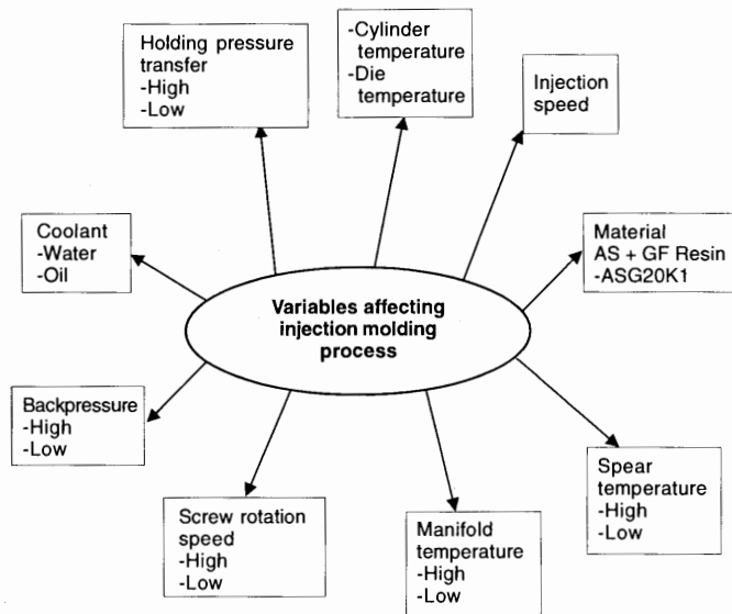
Figure 7 Variables affecting injection molding process
