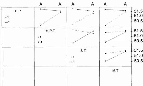
Figure 11 Interaction plot for analysis A
