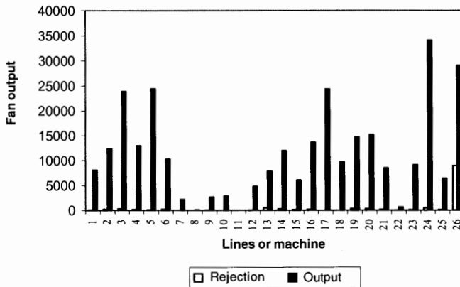
Figure 2 Total cross flow fan rejection for the month of December 2001 [4]
